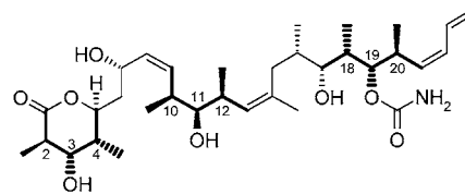
discodermolide ( 1 )
